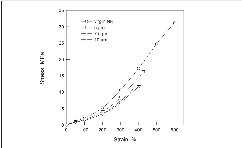
Figure 18.8: Stress-strain curves for 35 phr carbon black filled virgin NR and devulcanized NR devulcanized in a coaxial reactor at a flow rate of 0.63 g/s and various ultrasonic amplitudes. Gap = 2.54 mm, barrel temperature = 120°C.
