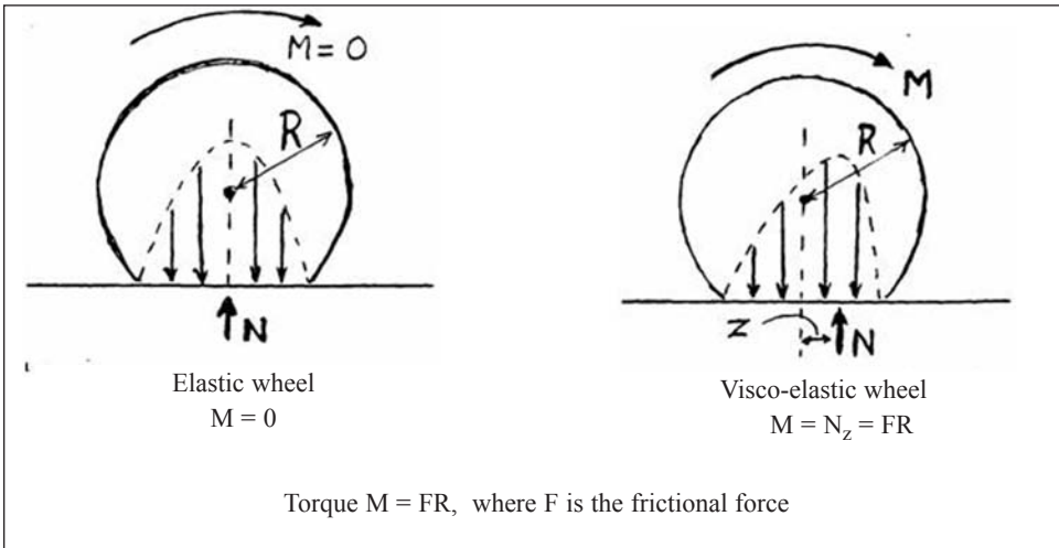
Figure 2.36: Rolling friction
