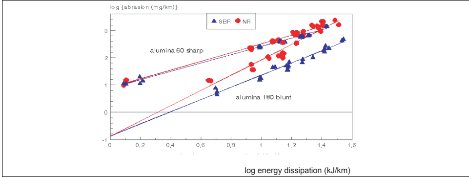
Figure 13.33: Log (abrasion) for two tread compounds NR + black and SBR + black on two surfaces of different sharpness: alumina 60 and alumina 180 (blunt) as a function of log (energy dissipation) [from ref. 31]
