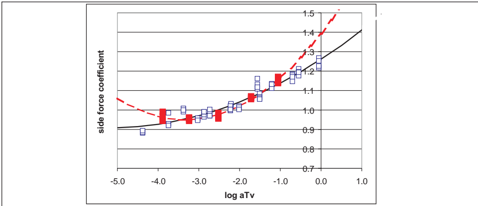
Figure 11.44: Side force coefficient of compound A (an OE-SBR black filled tire tread compound) on wet blunt alumina 180 as a function of \log a_{TV} obtained at three speeds and five temperatures (open squares) with a quadratic equation fitted to the data (black solid line). The red marked points were obtained at one speed for five temperatures with the dotted red line the best-fit quadratic equation, showing the risk of extrapolating from a limited set of data.
