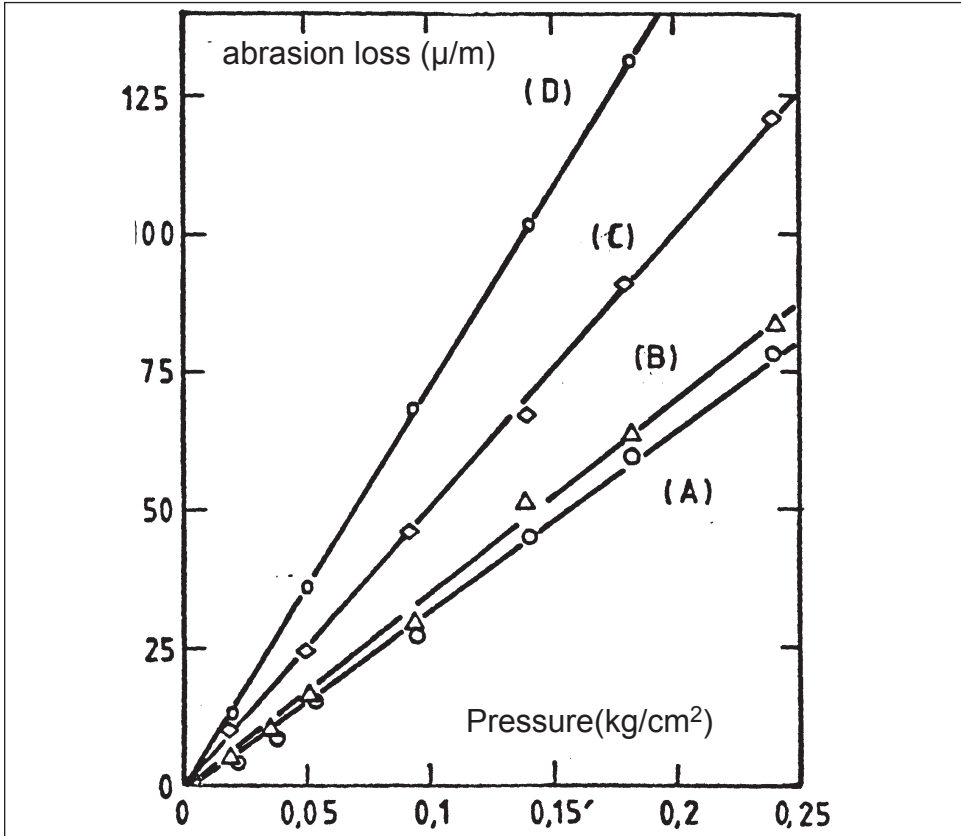
Figure 13.4: Abrasion loss as function of pressure for four different compounds [from ref .7] A, SBR+50 HAF black; B, NR +50 HAF black; C, NR+50 thermal black; D, NR+50 activated CaCO 3
