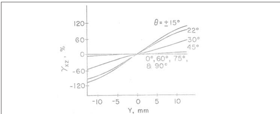
Figure 4.14 - Interlaminar shear strain ( \gamma_{xz} ) vs. position along specimen width for E_x = 20\% [20].
