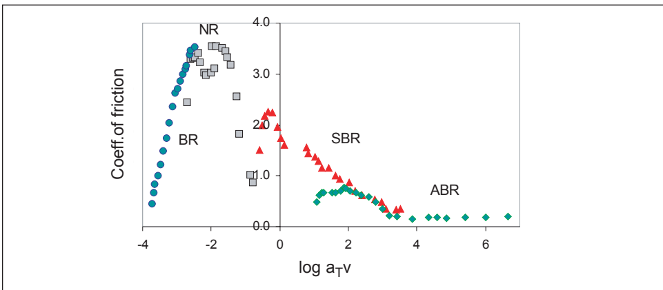
Figure 11.20: Friction coefficients of the four unfilled compounds of figure 19 plotted vs. \log a_T v [data from ref 34]
