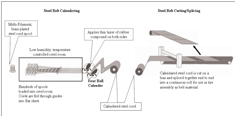
Figure 1.15: Tire manufacturing - steel stabilizer ply preparation
